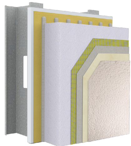
StoTherm® ci with Lancaster Nickel Metallic
